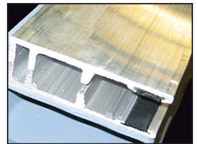
NYLON SIDE GUIDE STRIPS Eliminate metal to metal contact with slats.
